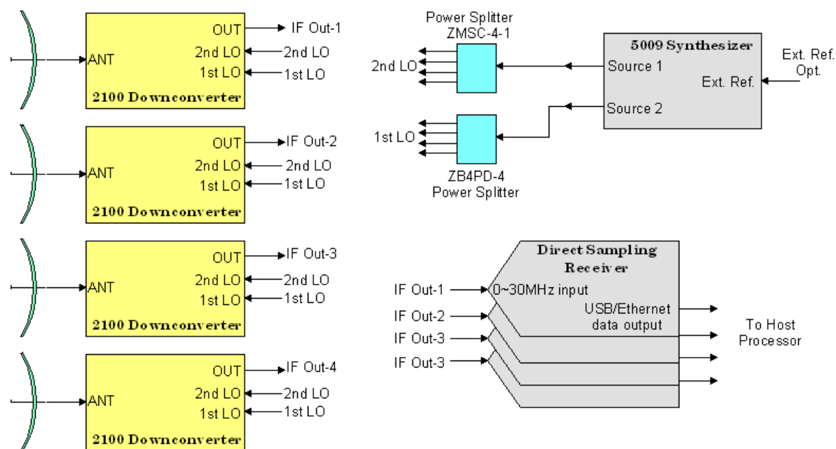
Figure 4 Small radio astronomy interferometer
