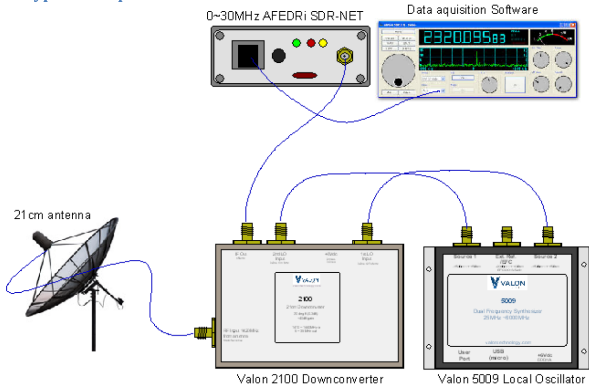
Figure 3 Typical downconverter connections using a Valon 5009 Dual Frequency Synthesizer.
