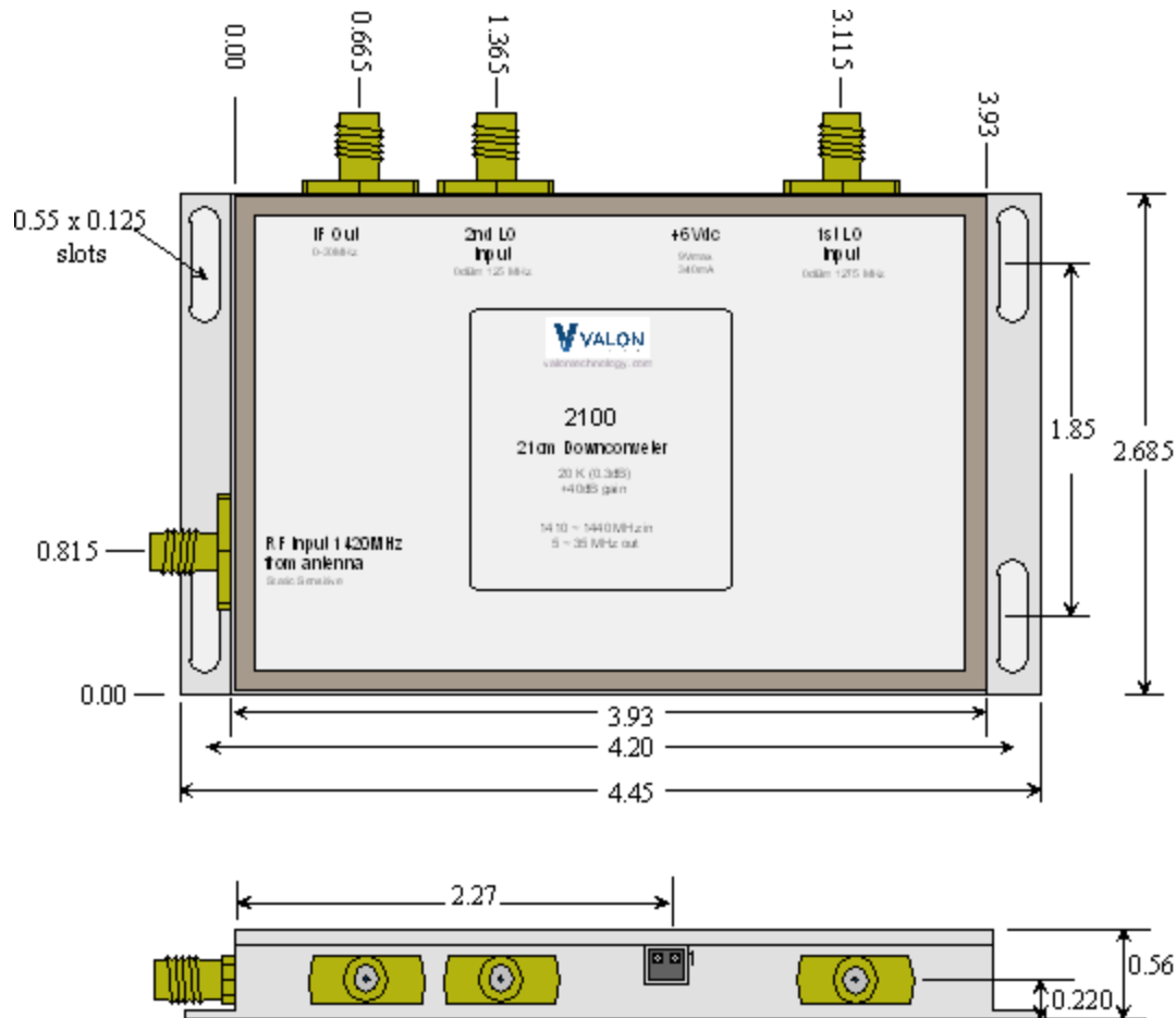
Figure 2 2100 module housing dimensions and mounting details.
