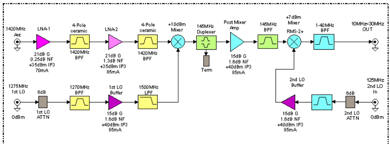
Figure 1 Block Diagram
